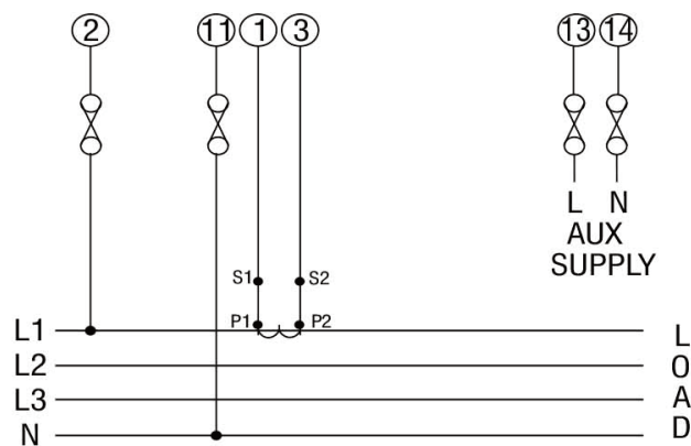
c) Single Phase Load
